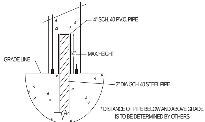
ANCHOR STYLE B
