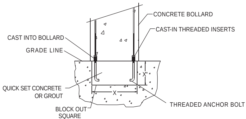
ANCHOR STYLE A
