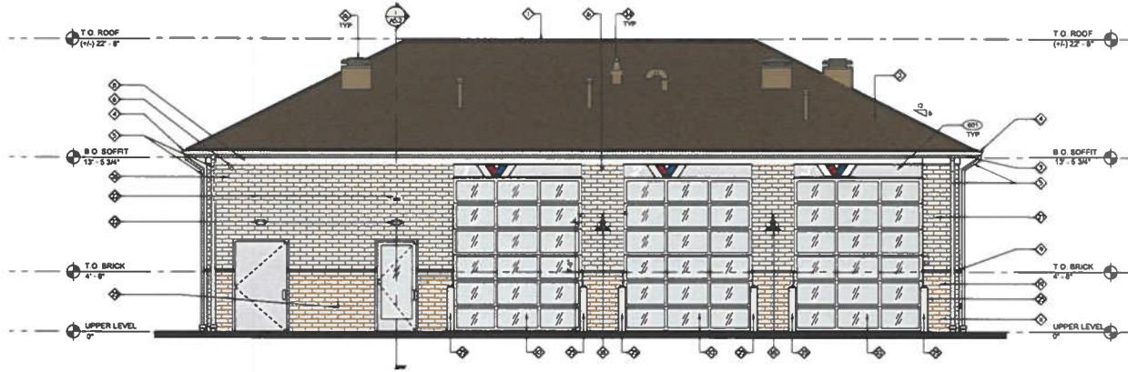
1 EXTERIOR ELEVATION SCALE 1/4" = 1'-0"
