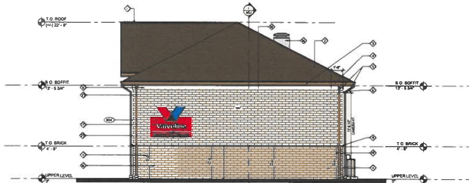
2 EXTERIOR ELEVATION SCALE 1/4" = 1'-0"
