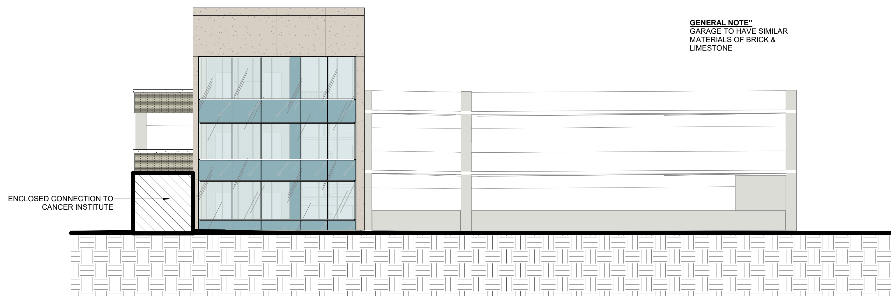
1 GARAGE NORTH ELEVATION 3/32" = 1'-0"
