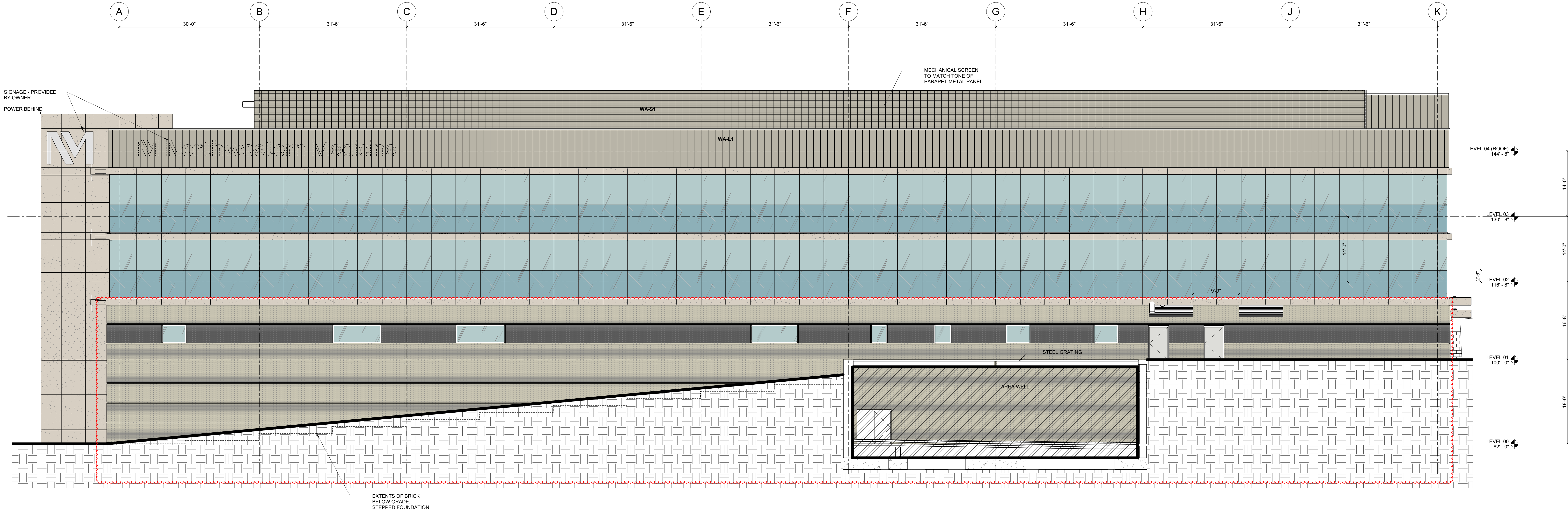
1 NORTH ELEVATION 1/8" = 1'-0"
