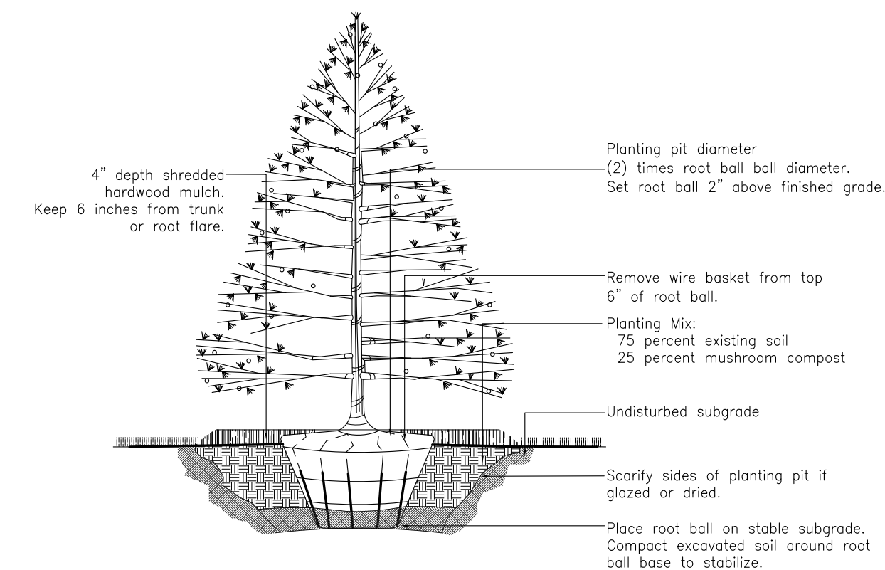
Detail Evergreen Tree Planting
