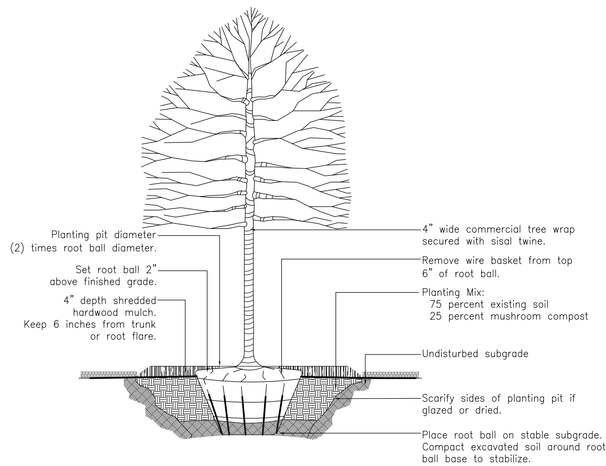
Detail Deciduous Tree Planting
