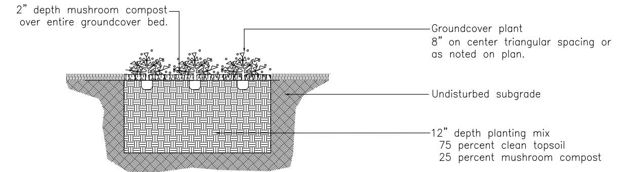
Detail Groundcover Planting
