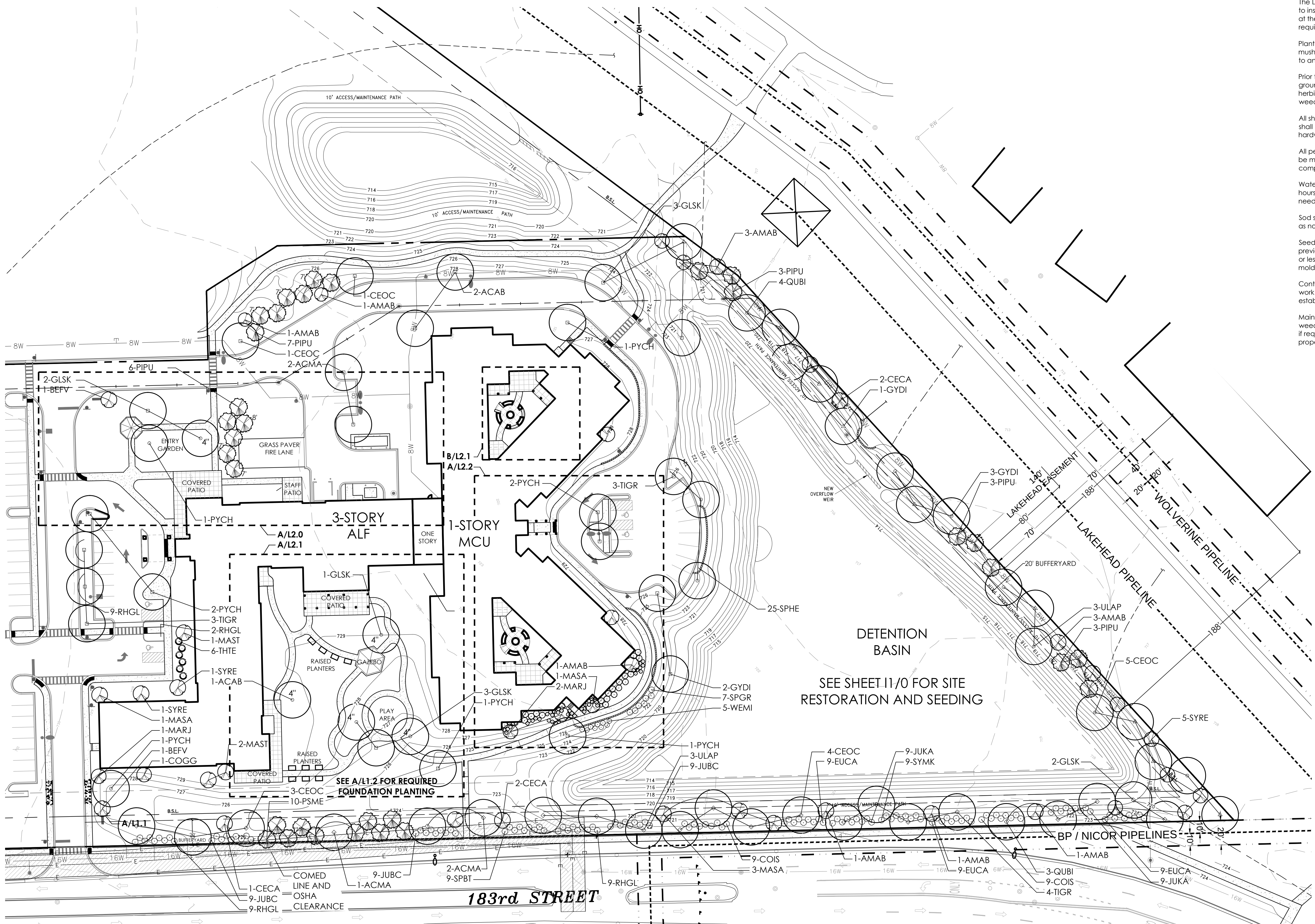
A SITE LANDSCAPE PLAN
