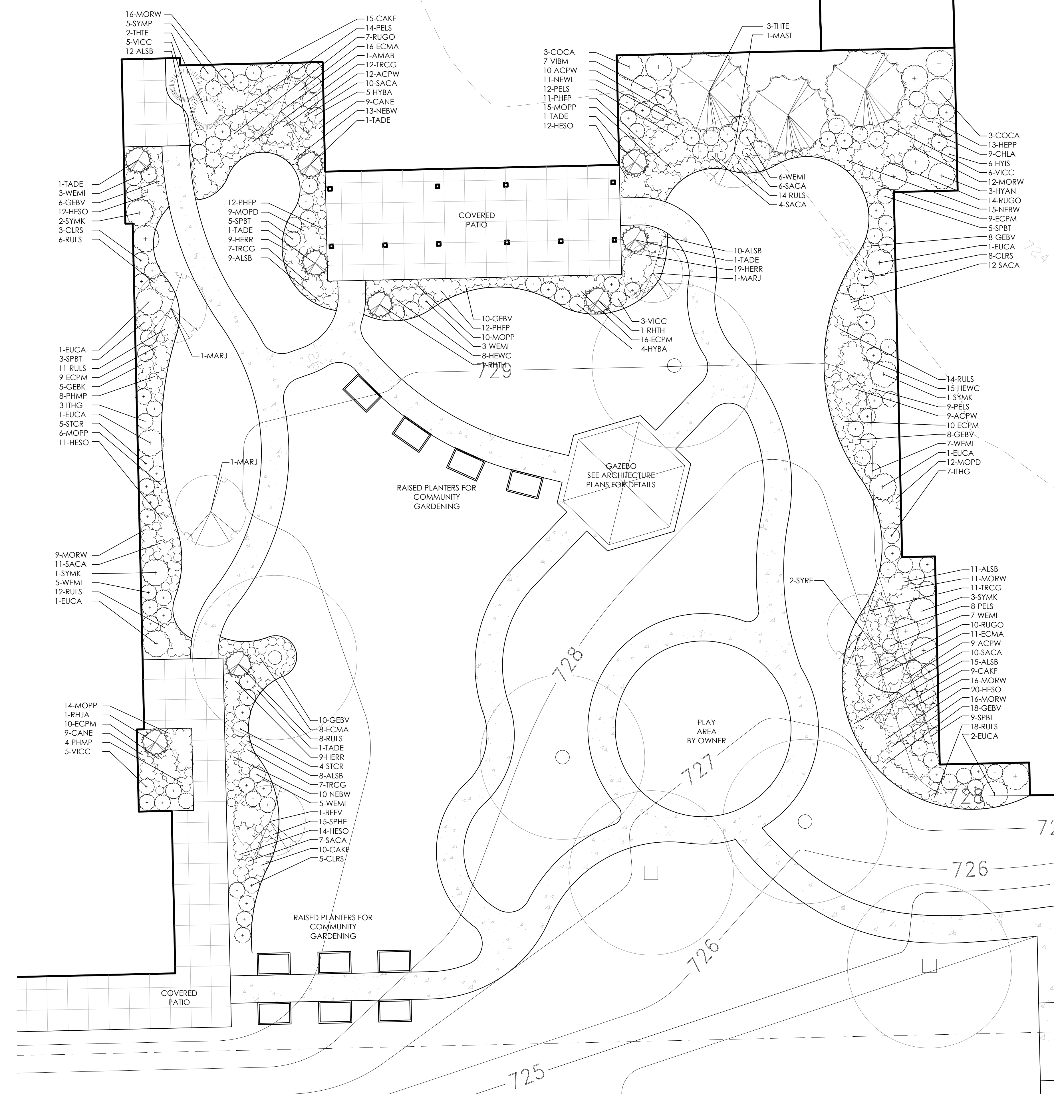
A ALF COURTYARD & PATIO PLANTING SCALE: 1" = 10'-0"
