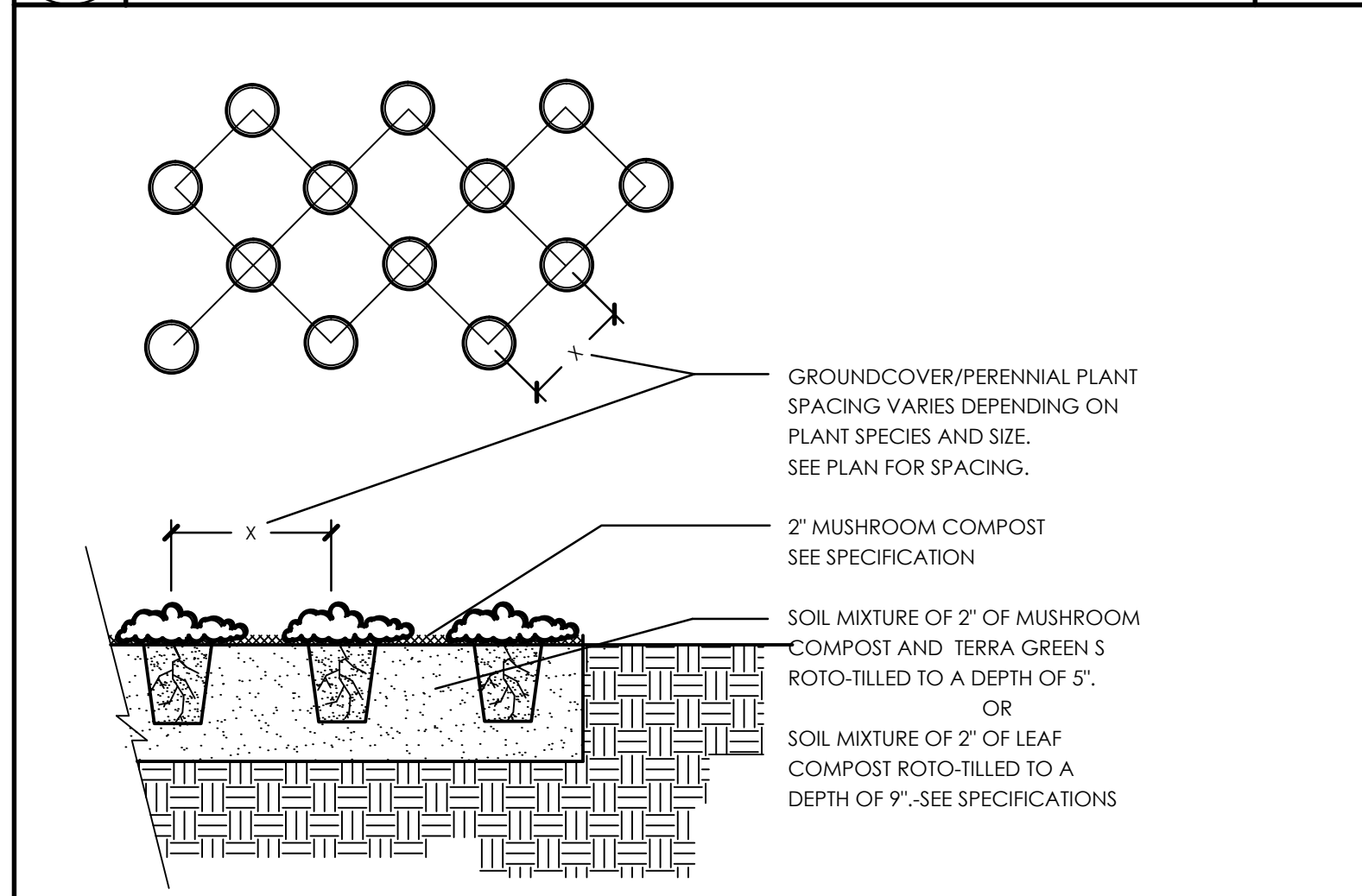
D PERENNIAL PLANTING DETAIL N.T.S.
