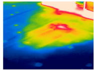
Thermogram T-01
