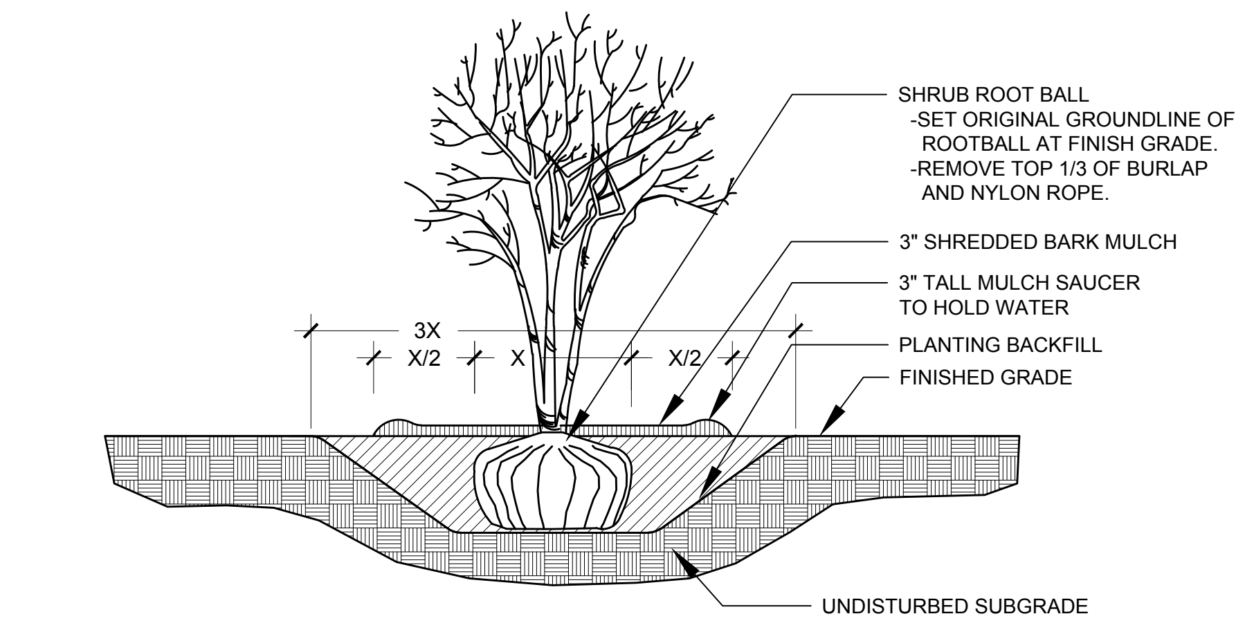
2 SHRUB AND ORNAMENTAL TREE PLANTING DETAIL NTS
