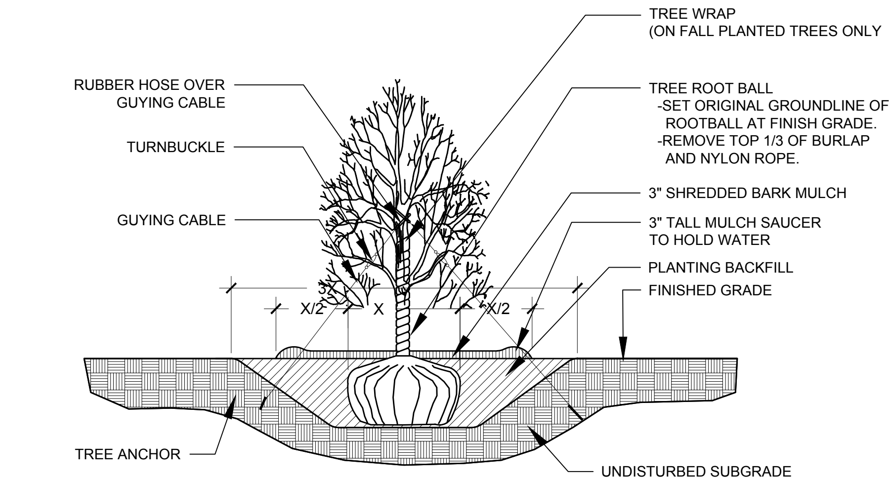
1 SHADE TREE PLANTING DETAIL NTS
