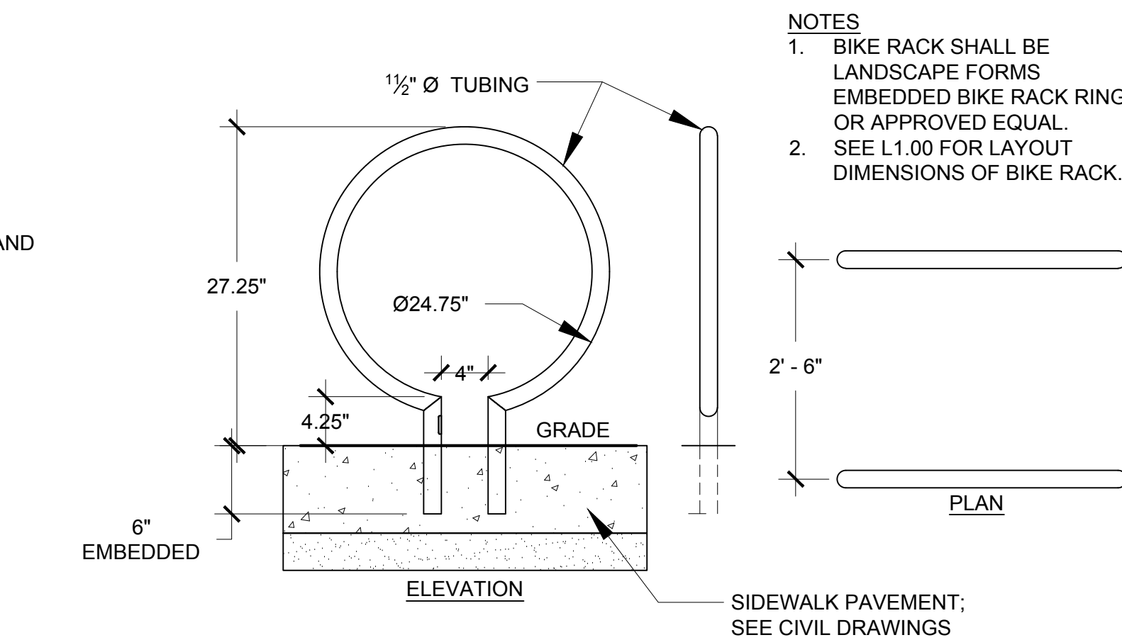
6 BICYCLE RACK DETAIL SCALE: 1\"/>
