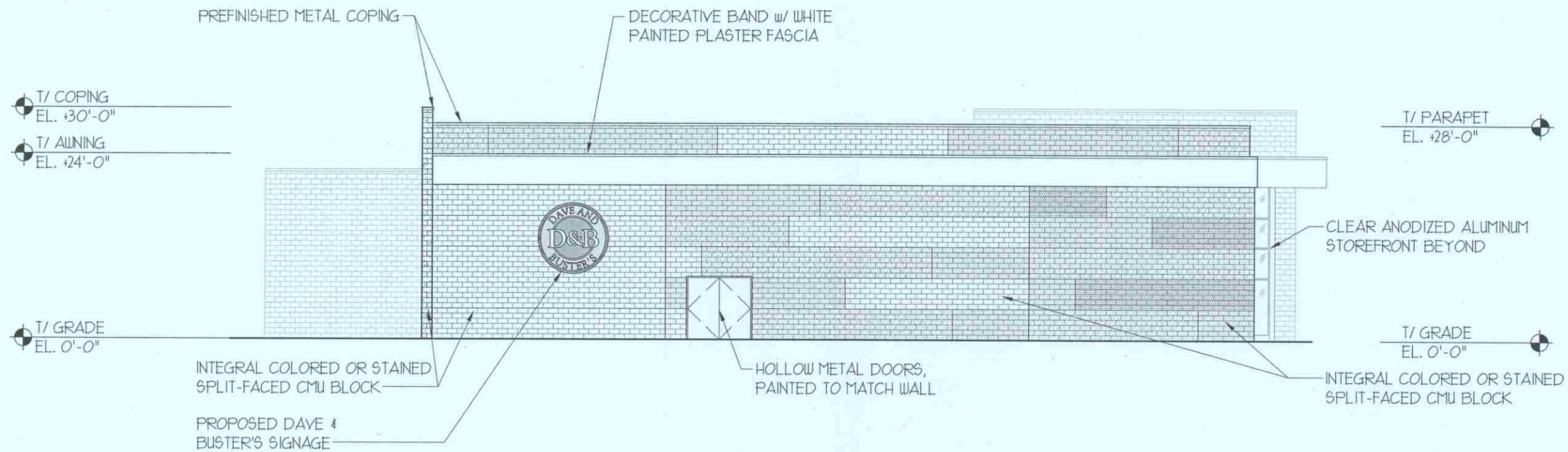
4 NORTH ELEVATION
