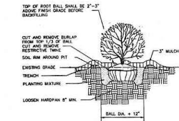
DETAIL: SHRUB PLANTING NOT TO SCALE
