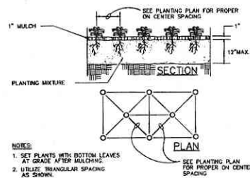
DETAIL: GROUNDCOVER PLANTING NOT TO SCALE
