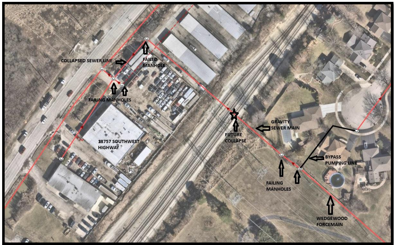
Wedgewood Forcemain Discharge Piping
