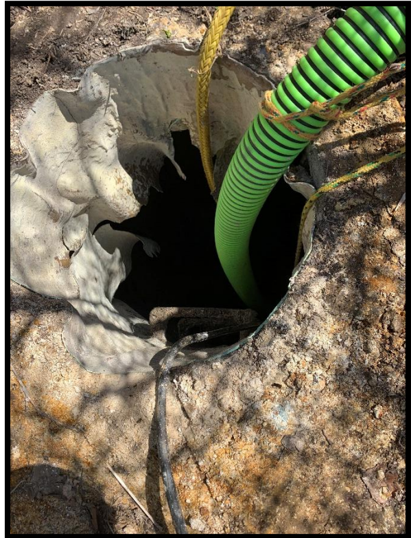
Epoxy Liner Failing
