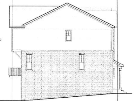
LEFT SIDE ELEVATION - 5-UNIT PLAN
