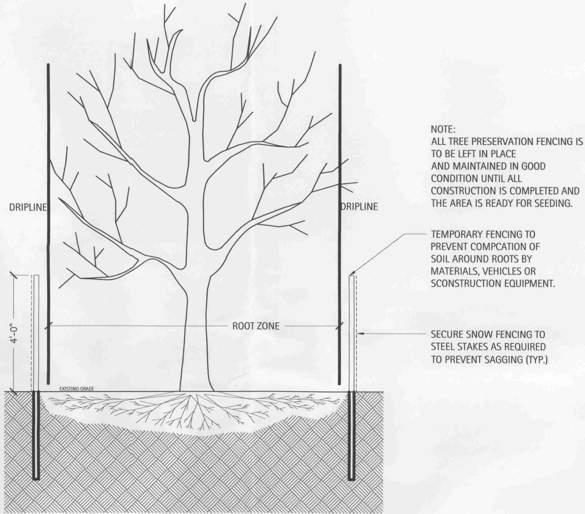
1 Tree Protection Detail Scale: NTS
