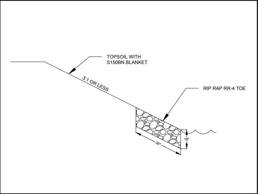
TYPICAL RIP RAP WRAP TOE ARMOR
