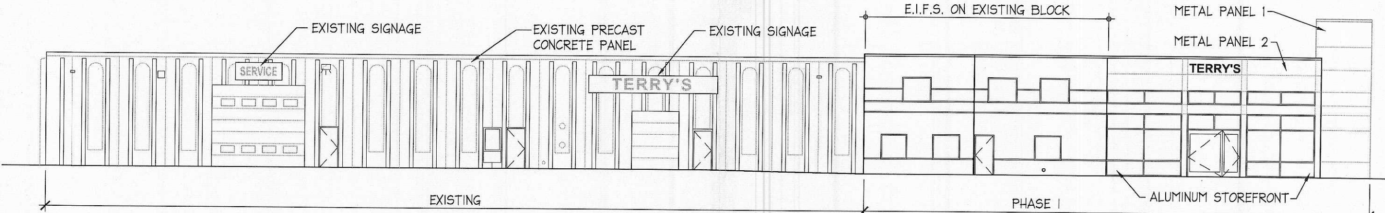
PROPOSED EAST ELEVATION 1/16"=1'-0"
