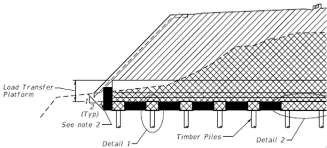
Figure 2- Cross Section showing load transfer platform
