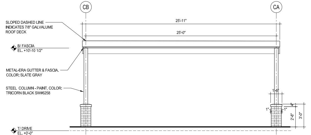
CREW CANOPY - SOUTH ELEV.
