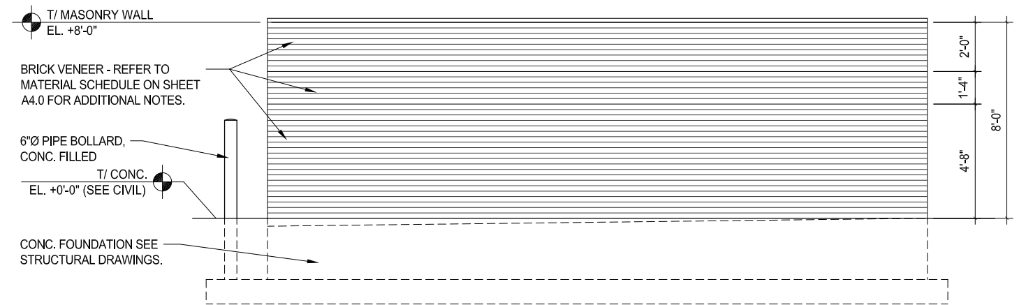
TRASH ENCLOSURE - SIDE ELEV.
