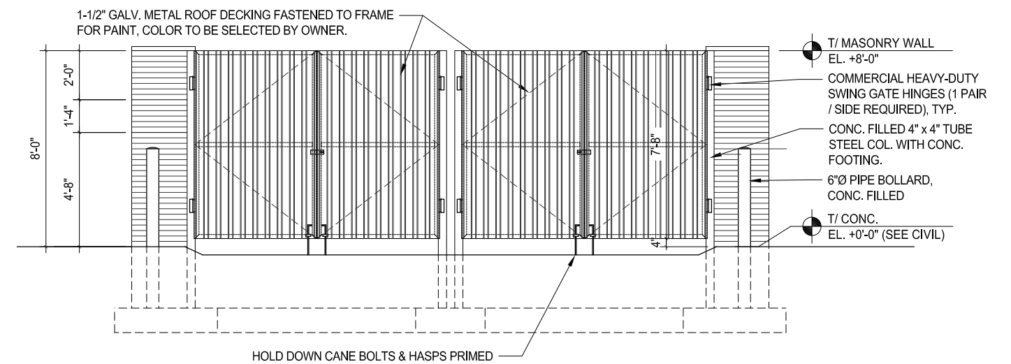
TRASH ENCLOSURE - FRONT ELEV.
