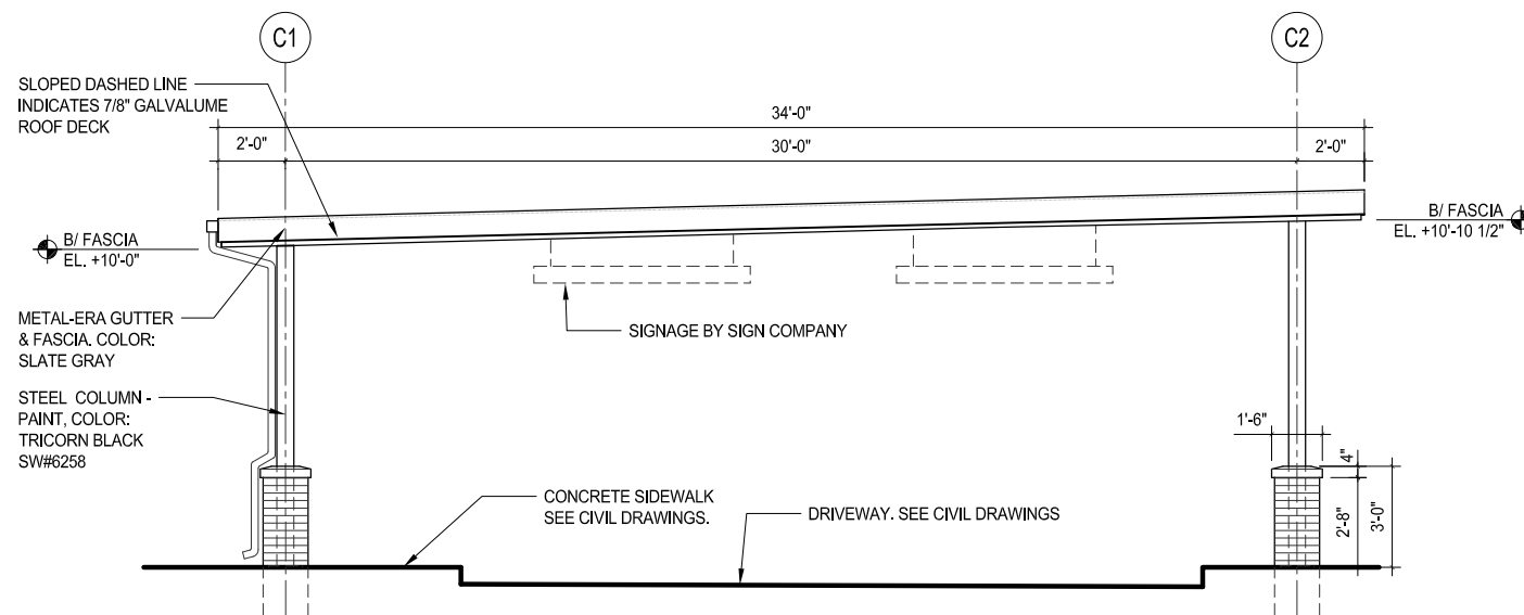
CREW CANOPY - WEST ELEV.
