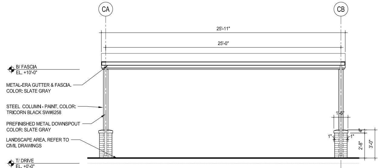
CREW CANOPY - NORTH ELEV.
