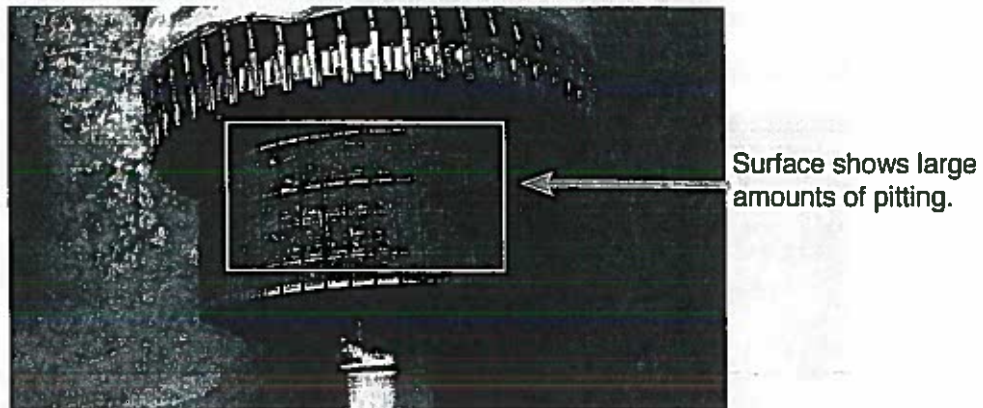
Figure 28 Commutator Wear
