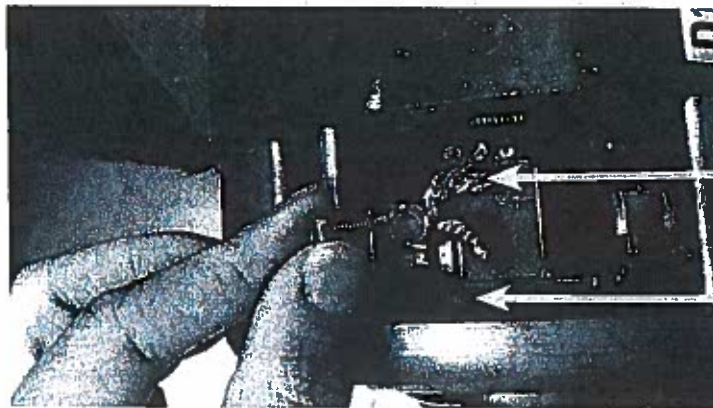
Figure 29 Replacing Brush Shunt Bolt
