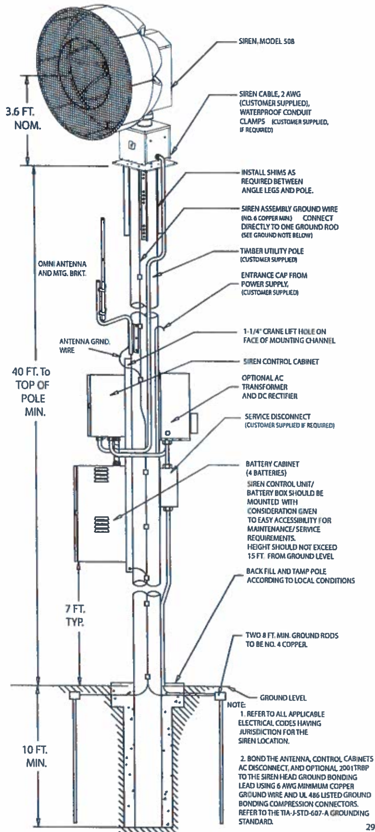
Figure 3 Typical Pole Installation (Model 508-128 shown)
