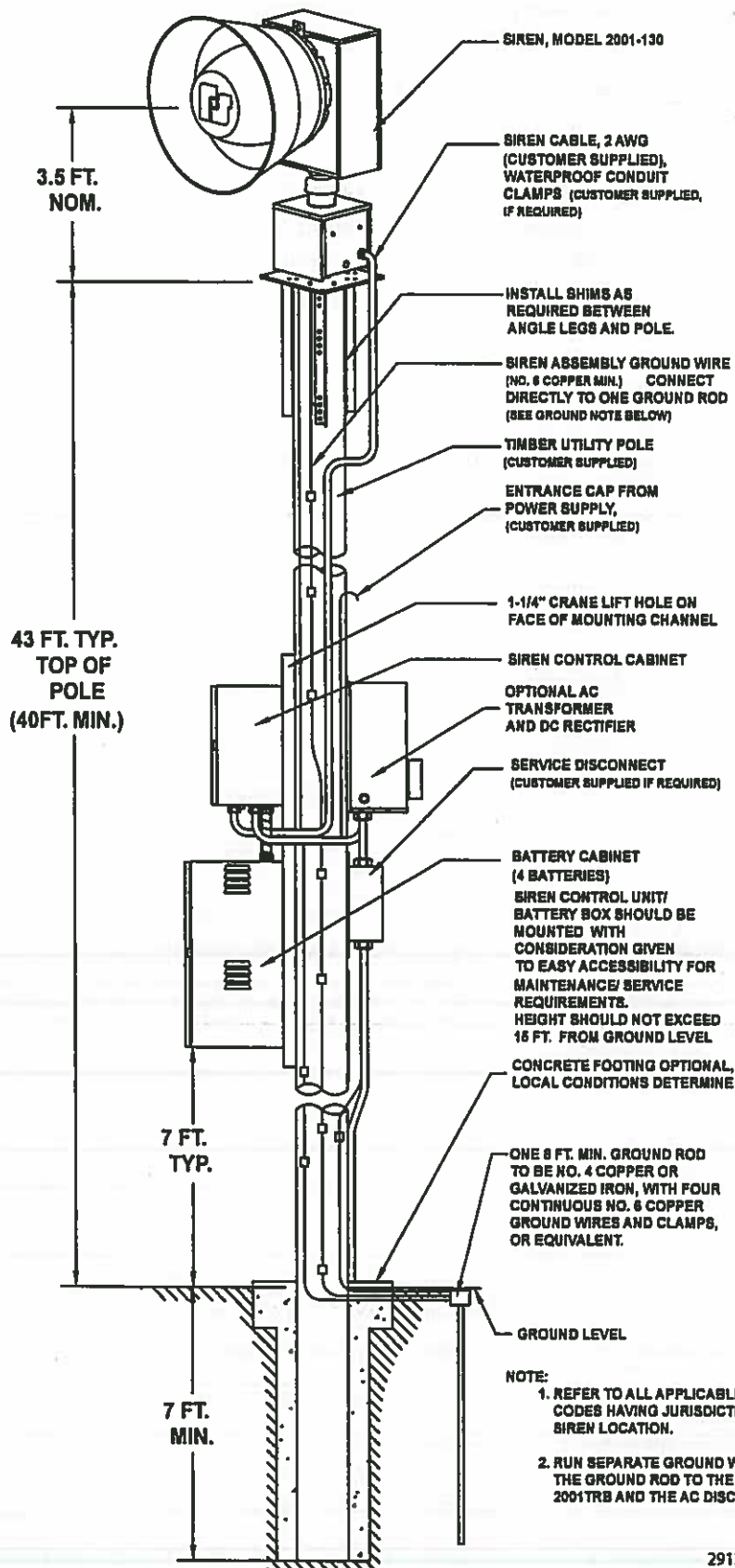
Figure 4 Typical DCFCB or DCFCTB with 2001TRBP Installation Drawing
