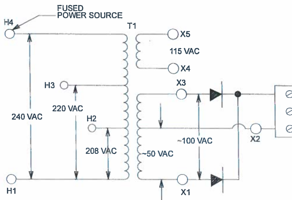
Figure 8 Schematic Diagram 2001TRBP
