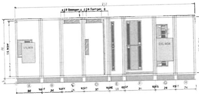
ELEVATION VIEW
