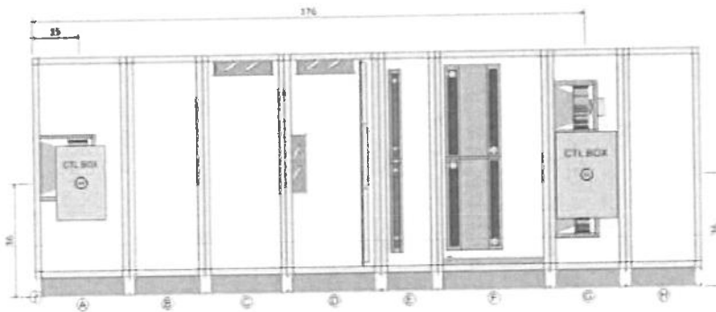
RIGHT ELEVATION VIEW
