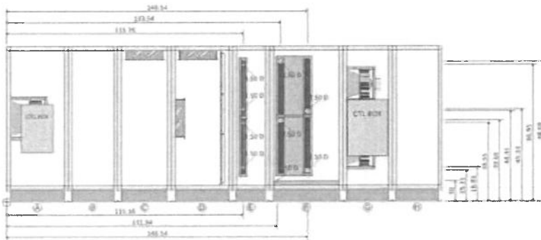
RIGHT ELEVATION VIEW
