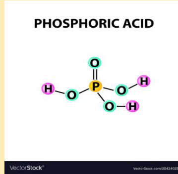
Phosphoric Acid
