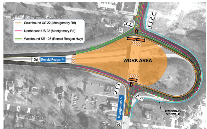
Temporary traffic pattern during Phase 2 of construction. This traffic pattern was in place for most of construction.
