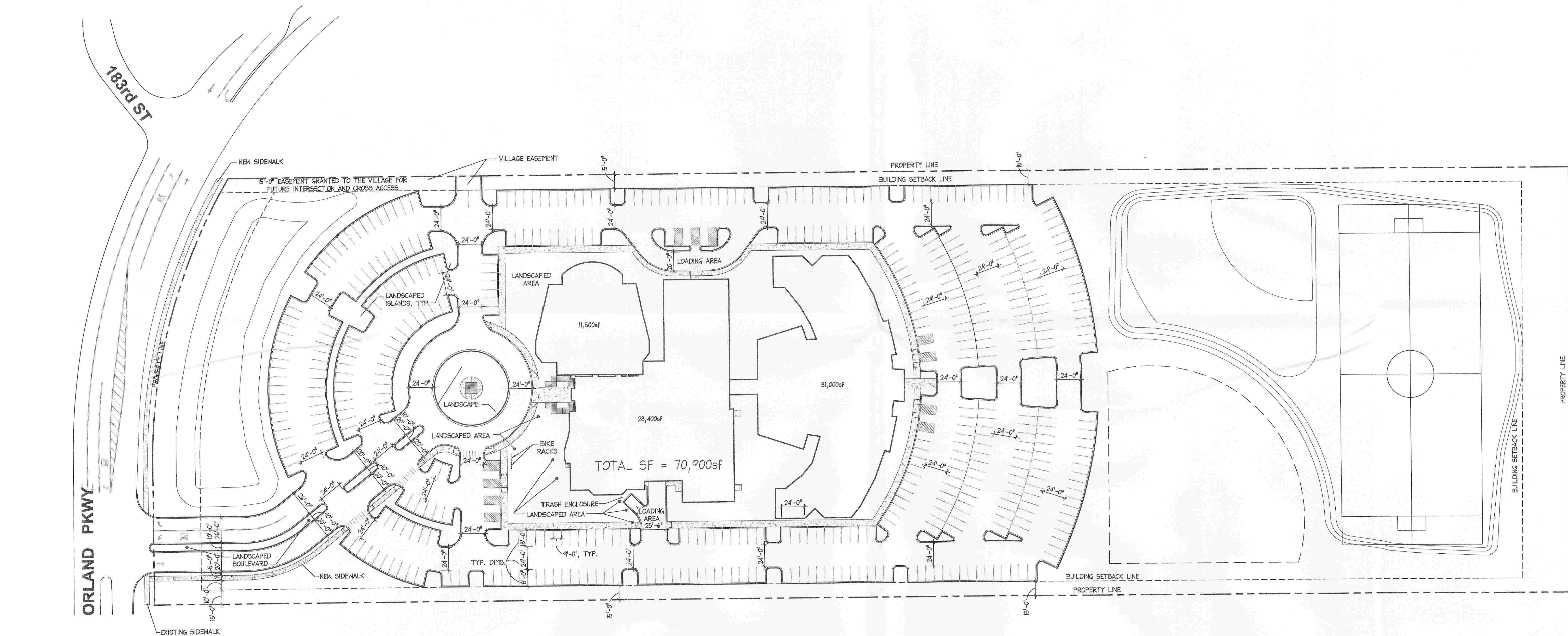
SITE PLAN - PHASE 1 & PHASE 2 1" = 50'-0"
