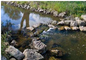
► Example of cross vane weir in channelized stream with 2:1 vegetated slope
