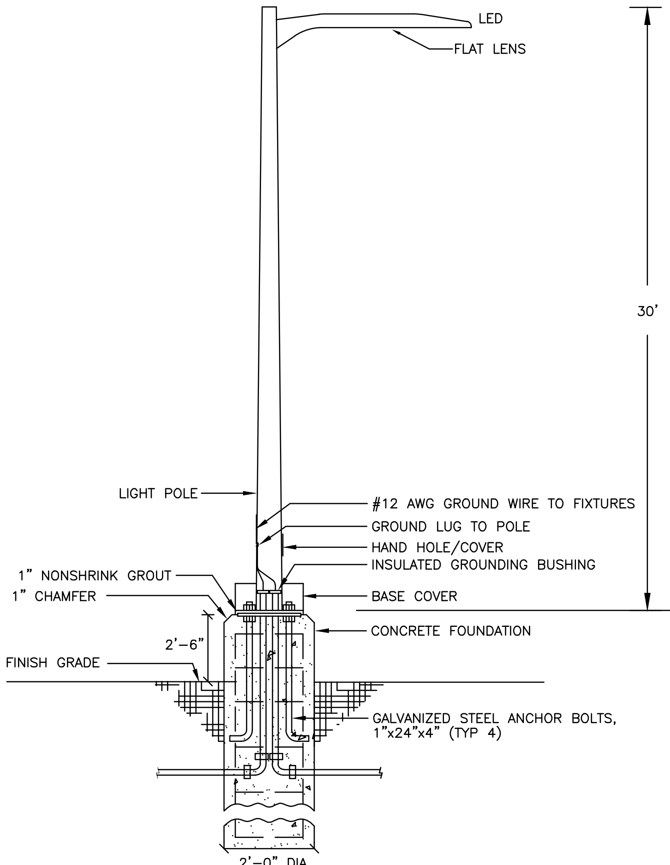
POLE BASE DETAIL NO SCALE
