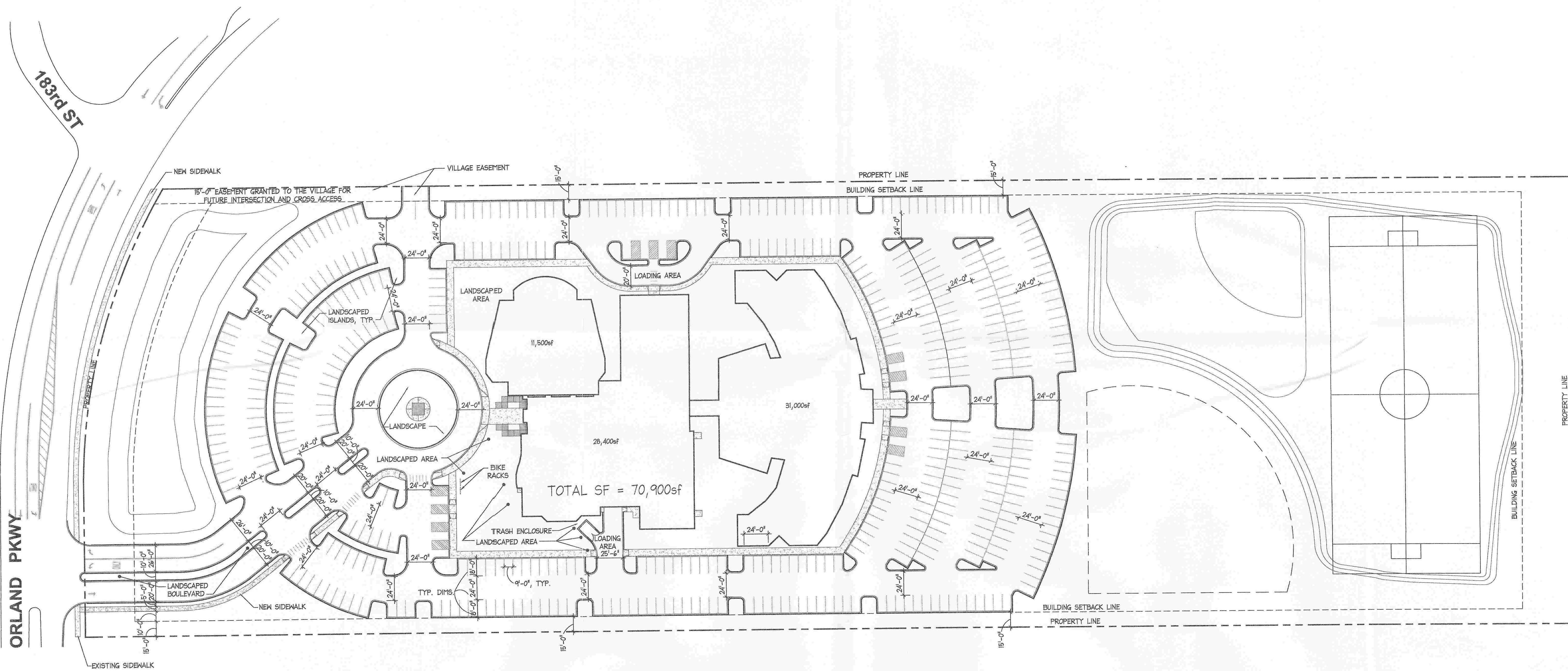
SITE PLAN - PHASE 1 & PHASE 2 1" = 50'-0"
