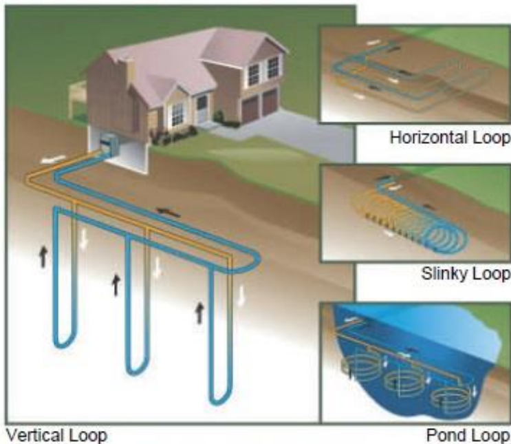
Figure 1: Geothermal energy system types include: 1) Vertical loop systems that reach deep into the earth; 2) Horizontal loop systems that stay near the surface but are below the frost line; 3) Slinky loop systems that maintain a moderate depth and increase the length/ capacity of the system on a compact lot; 4) Pond loop systems that sink geothermal cables into detention ponds; and 5) Open loop systems (not pictured) that are cables in the ground.
