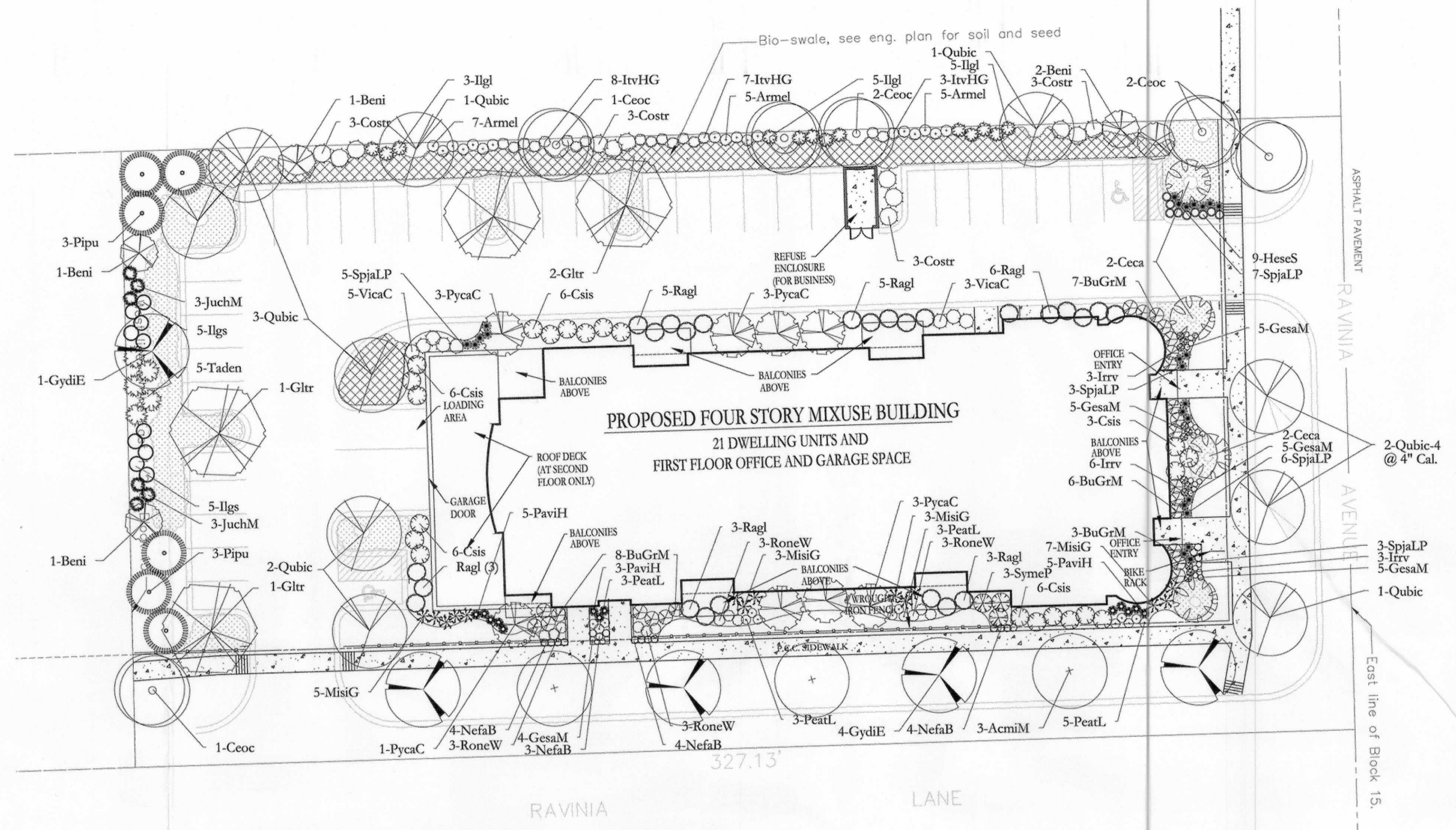
1 LANDSCAPE PLAN 1" = 20'
