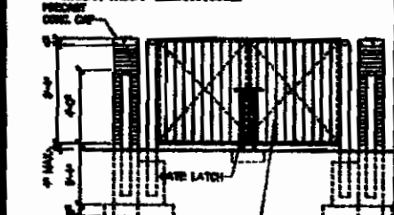
EAST/WEST ELEVATION
