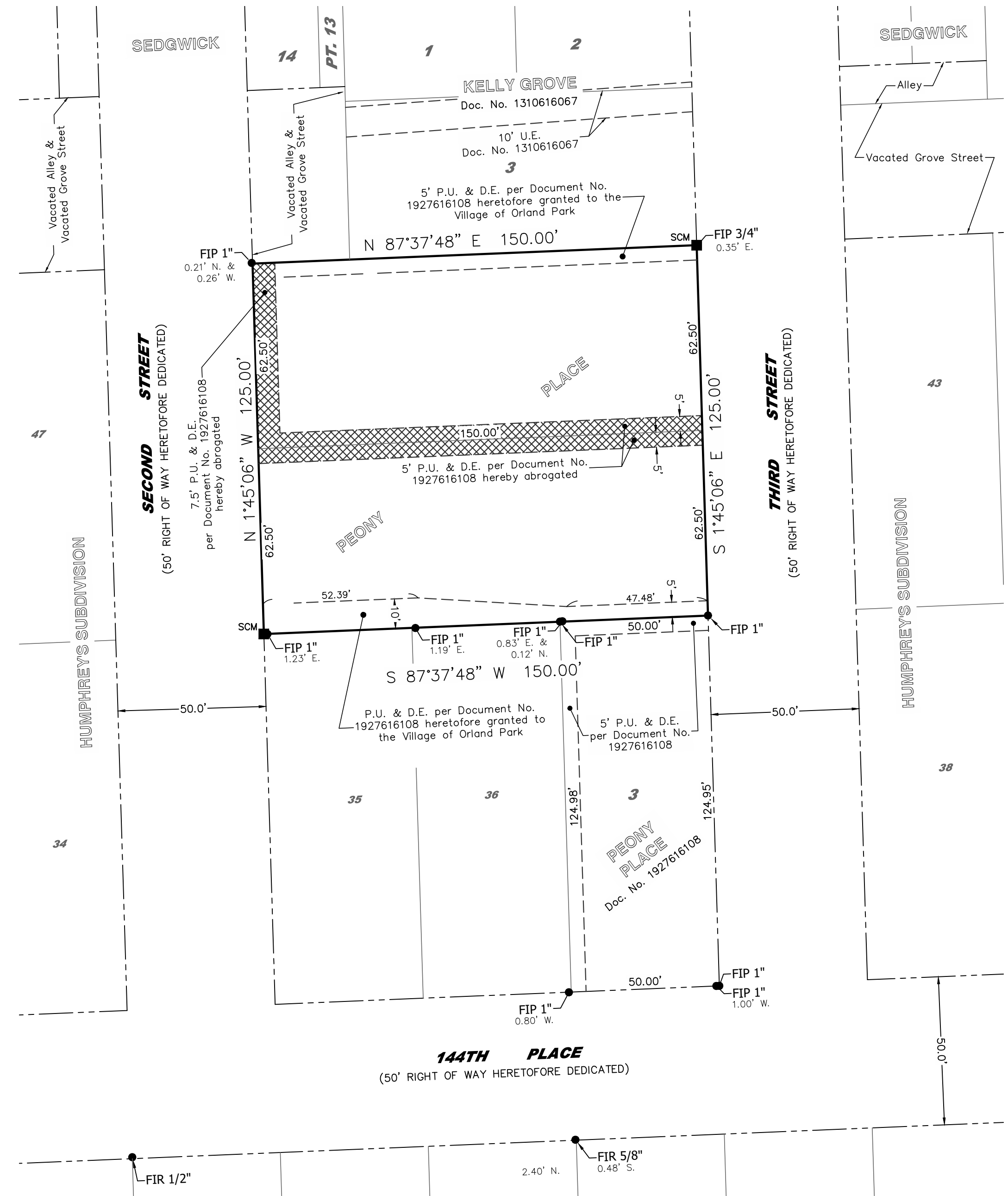
EXISTING CONDITIONS
