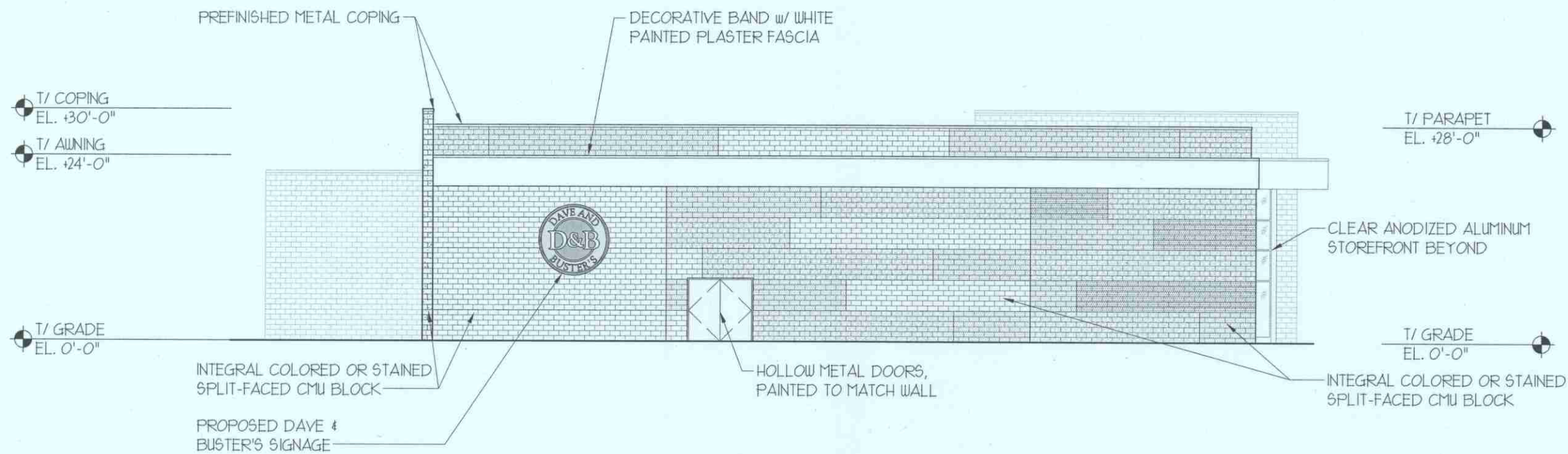
4 NORTH ELEVATION
