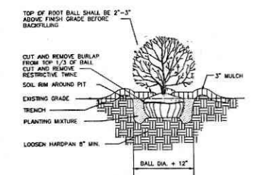
DETAIL: SHRUB PLANTING NOT TO SCALE
