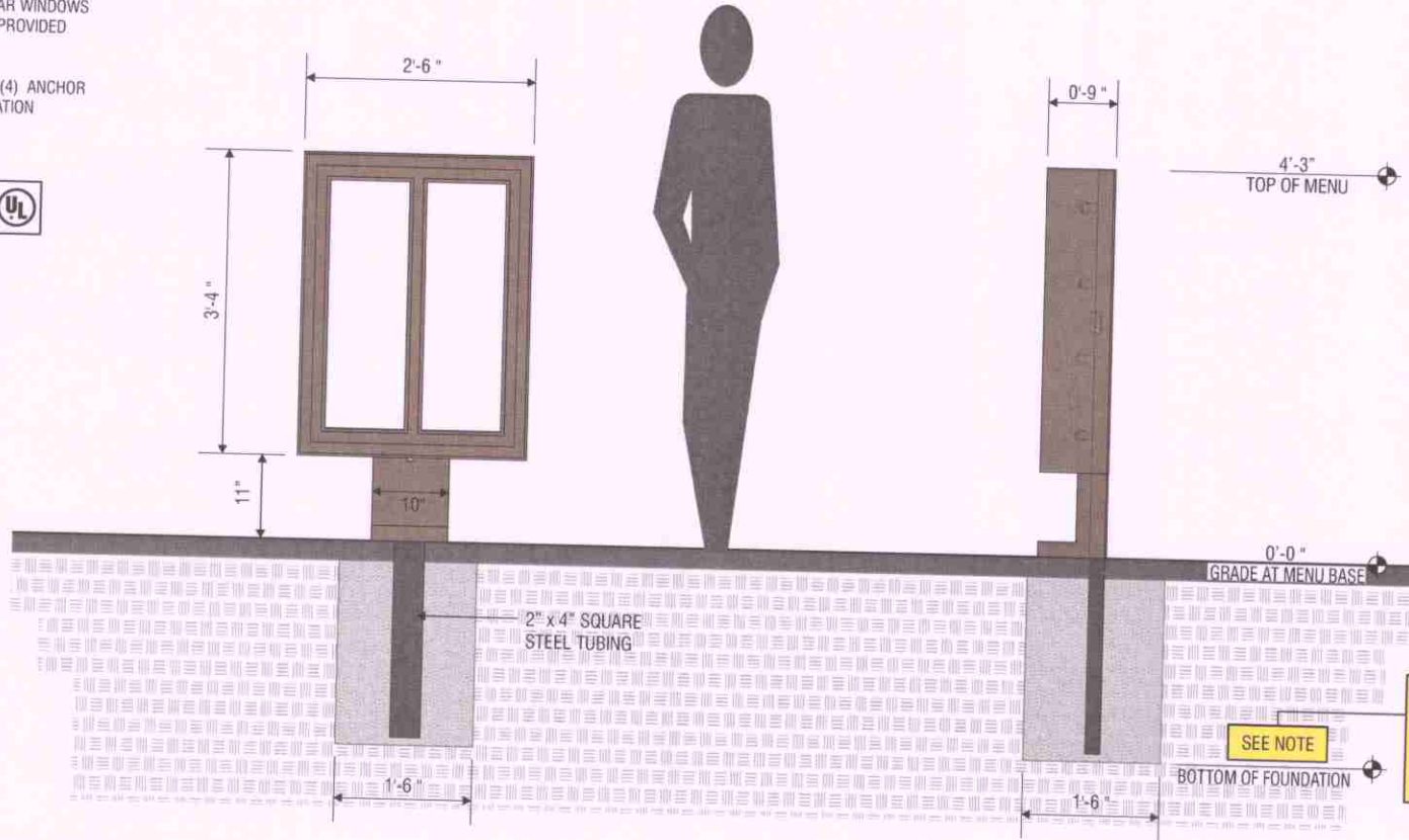
ELEVATION SCALE - 3/4" = 1'-0"
