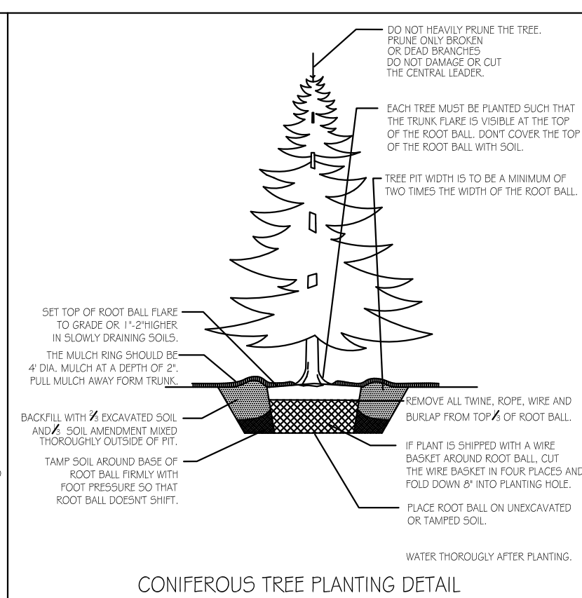
CONIFEROUS TREE PLANTING DETAIL
