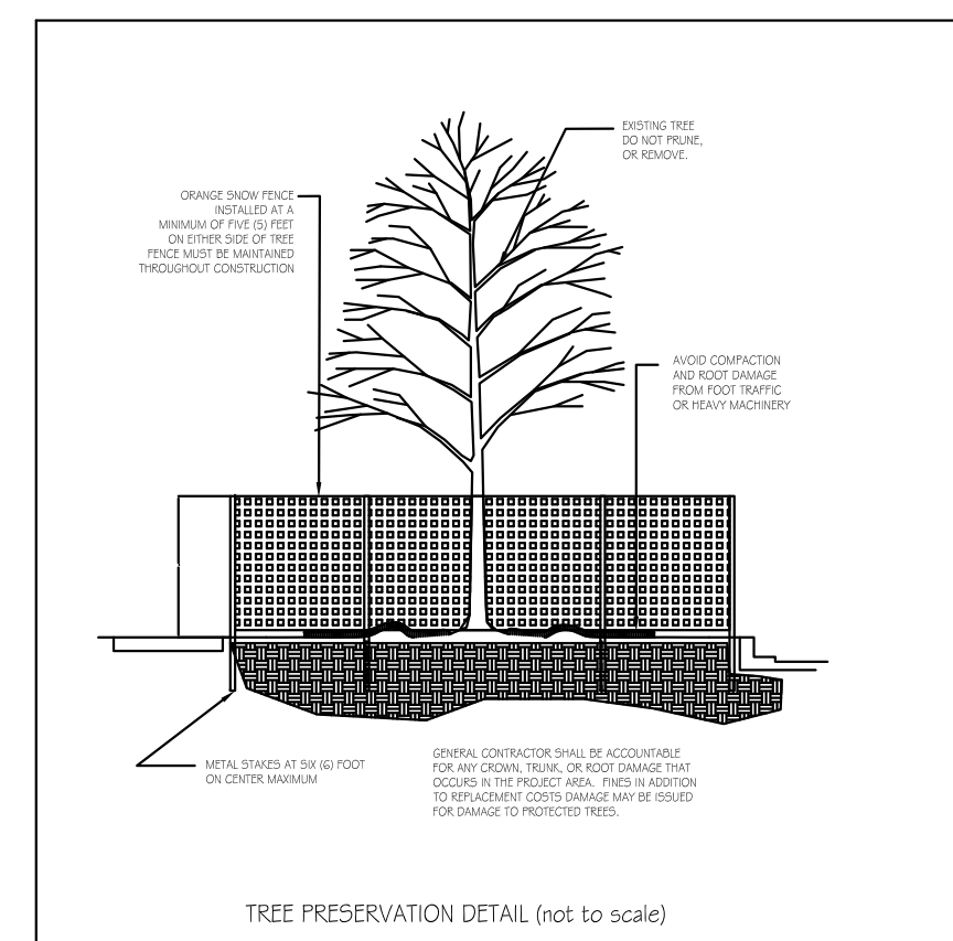
TREE PRESERVATION DETAIL (not to scale)
