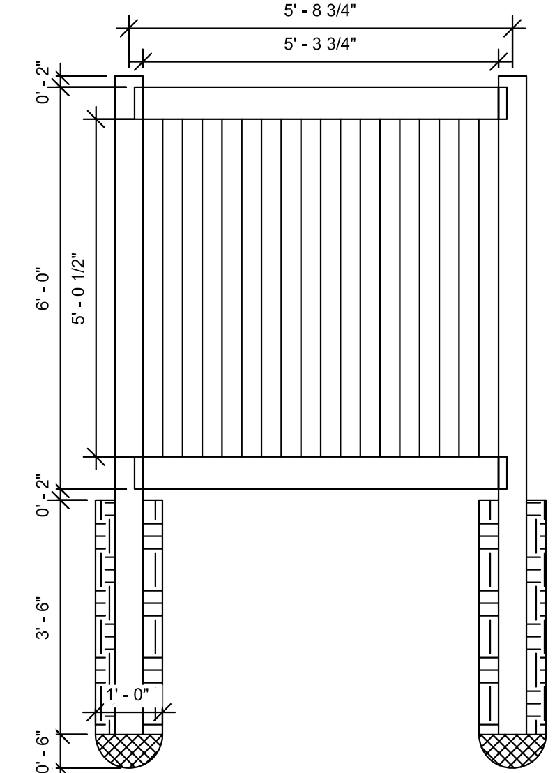
FENCE POST DETAIL 1/2" = 1'-0"
