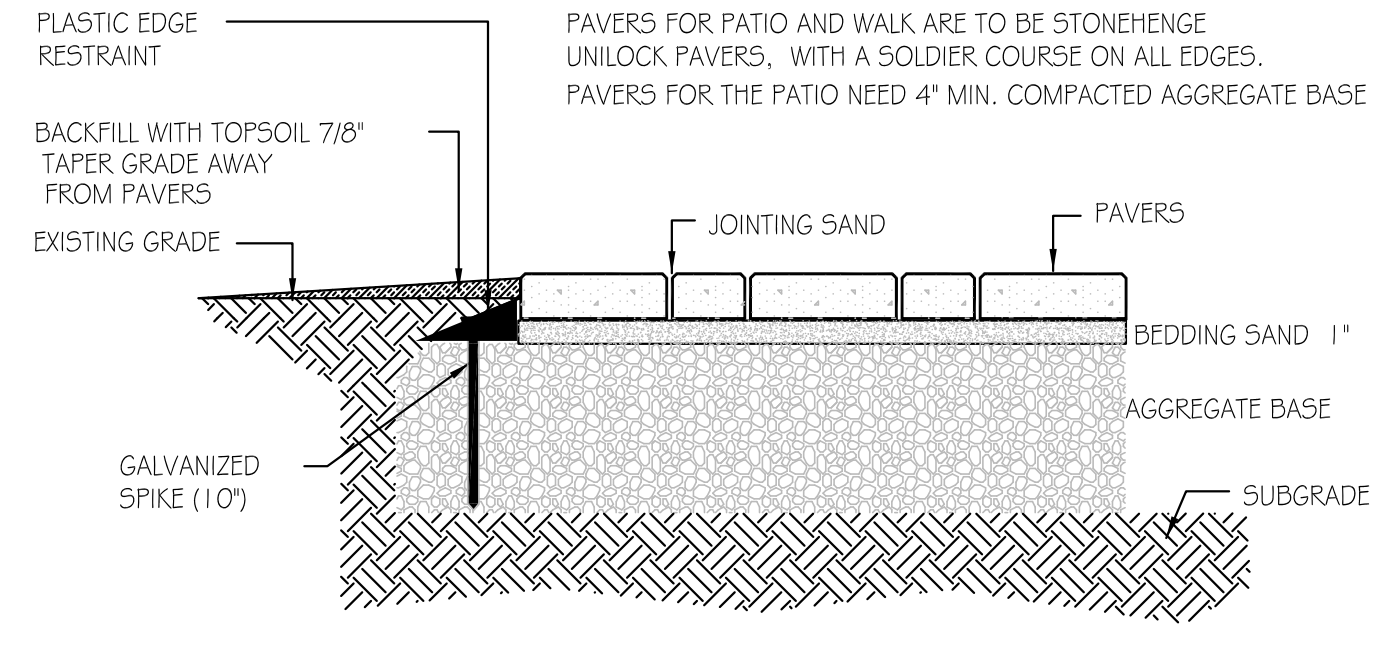
PAVER DETAIL 1/8" = 1'-0"
