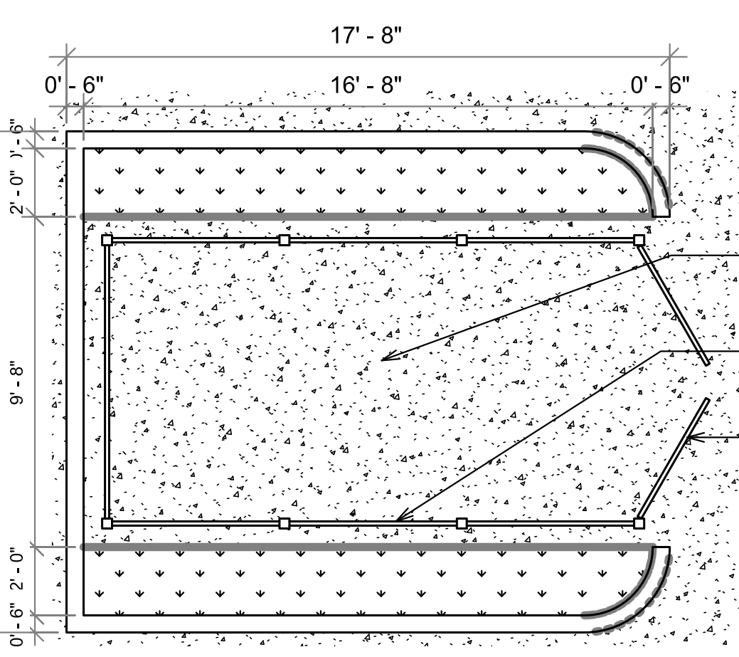
TRASH ENCLOSURE 1/4" = 1'-0"
