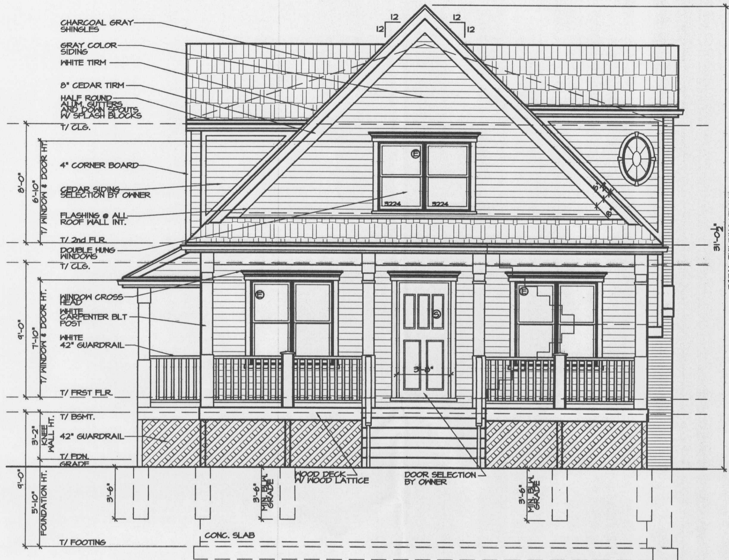
NORTH ELEVATION
